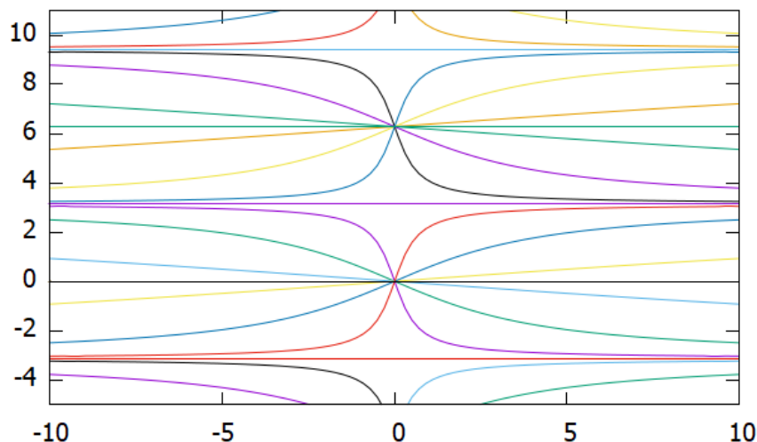
Figure 6: For Example 3.49: Several solutions of x \frac{dy}{dx} = \sin y , plotted in the rectangle -10 \leq x \leq 10 , -5 \leq y \leq 11 . (The displayed solution curves are maximal in this region.) The horizontal lines in the figure are the constant solutions y = -\pi , y = 0 , y = \pi , y = 2\pi , and y = 3\pi .
