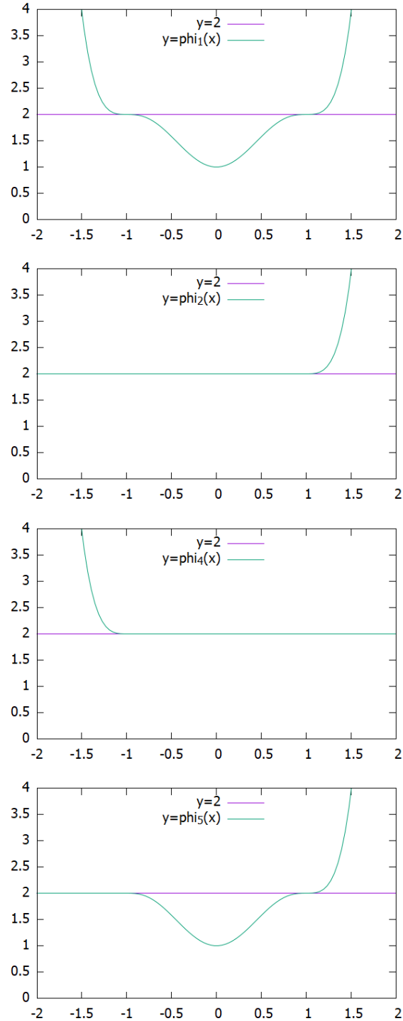
Figure 4: For Example 3.48: The solutions \phi_1, \phi_2, \phi_4 , and \phi_5 , plotted simultaneously with the constant solution 2. The coordinate axes (not shown) are the usual x and y axes. The graph of \phi_1 intersects the graph of the constant solution, but does not overlap it. The graphs of \phi_2, \phi_4 , and \phi_5 do overlap with the graph of the constant solution. The graph of \phi_3 (not shown) is the mirror image of the graph of \phi_5 .
